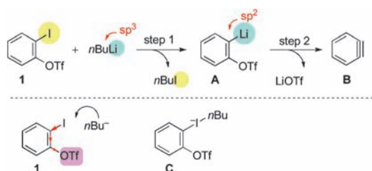
Scheme 1. Rapid benzyne generation. Tf = trifluoromethanesulfonyl.
