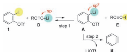
Scheme 2. Slow benzyne generation.
