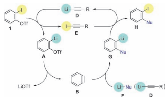
Scheme 3. Catalytic generation of benzyne and nucleo-iodination.
