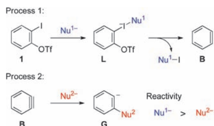
Scheme 5. Two roles played by nucleophilic species.
