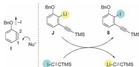
Scheme 4. Regioselectivity directed by an \alpha -alkoxy group.
